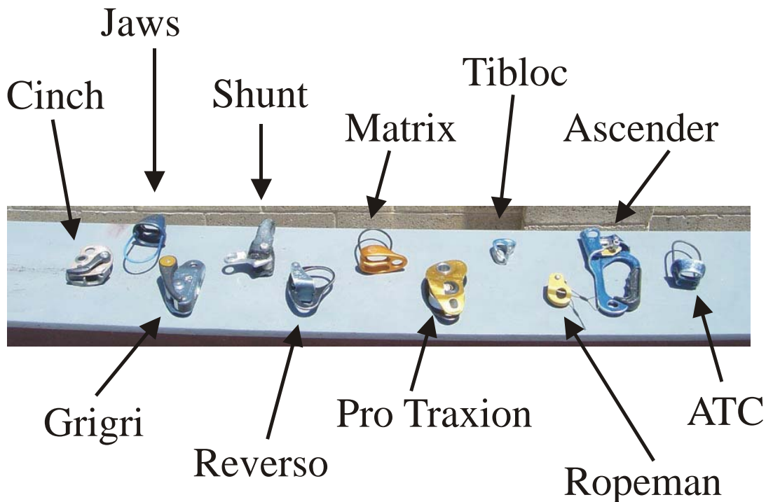
Figure 10: Different belay (both traditional and non-approved) devices tested
