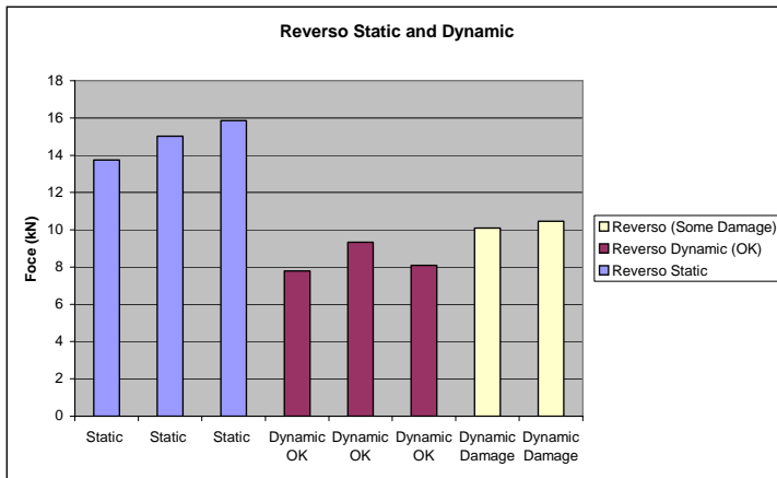
Figure 13: Static and dynamic results for a Reverso with a stopper knot.
