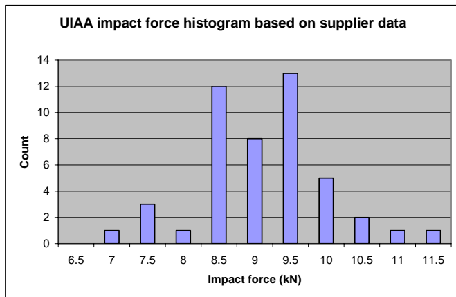
Figure 1: Histogram of rope UIAA impact force used to determine rope modulus.
