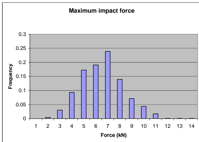
Figure 7: Creditable Lifetime Impact Fall Force (CLIFF) - Expected maximum fall force distribution based on climber weight, rope stiffness, and maximum fall factor distribution.
