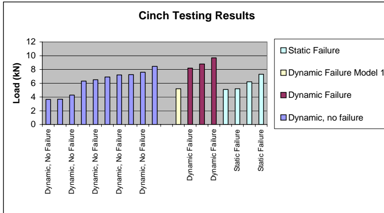
Figure 14: Static versus dynamic failure for Cinch.
