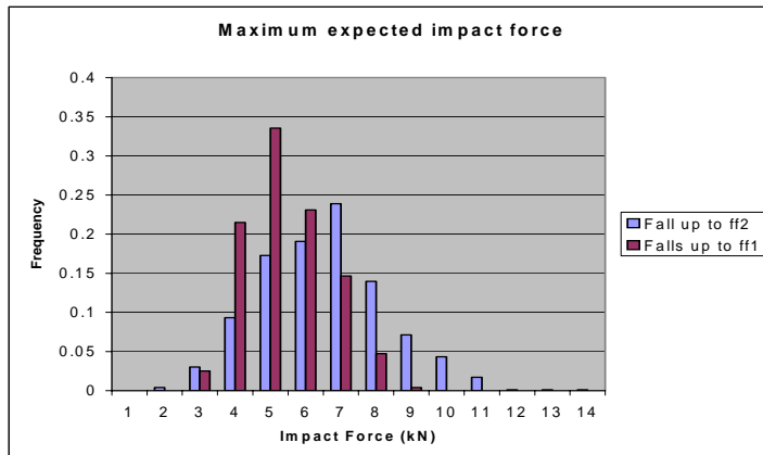
Figure 9: Maximum expected impact force for falls limited to fall factor 1.0 compared with impact force for all falls.
