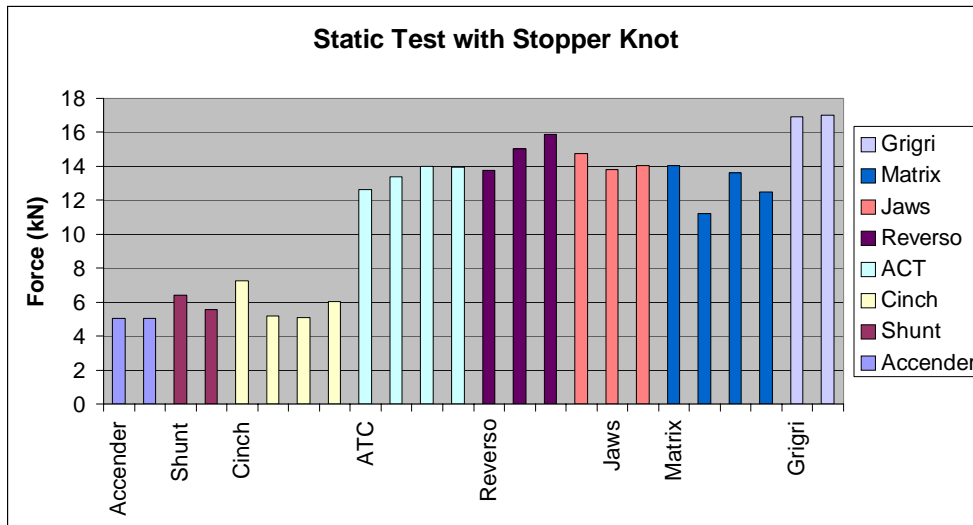
Figure 11: Static failure force for belay devices.
