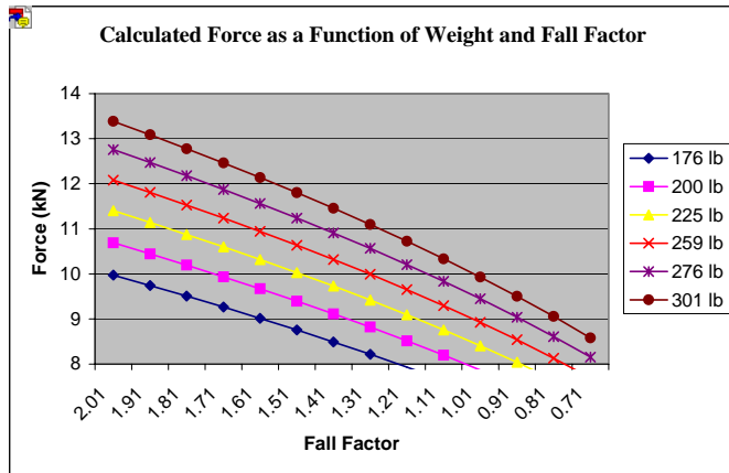
Figure 6: Calculated (impact) force as a function of weight and fall factor.
