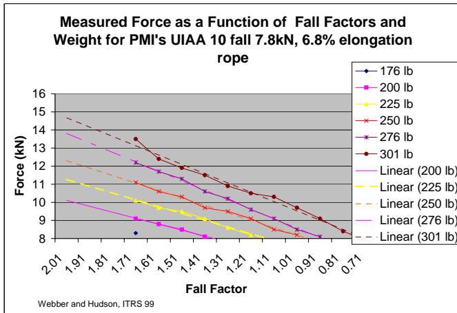
Figure 5: Force as a function of fall factor and weight. A linear (straight-line) approximation has been added to Webber and Hudson’s data to project the data to a fall factor of 2.0
