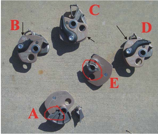
Figure 16: Dynamic (A, C, D, and E) and static (B) failure modes for belay devices were not always similar and repeatable. Shown here is the Cinch.
