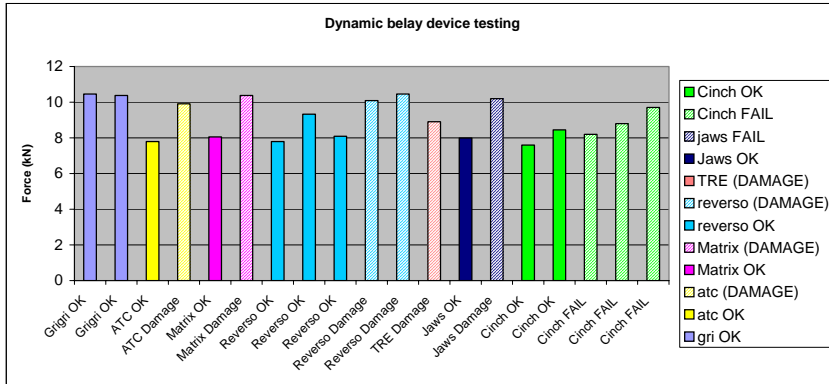
Figure 12: Dynamic Results for different belay devices.
