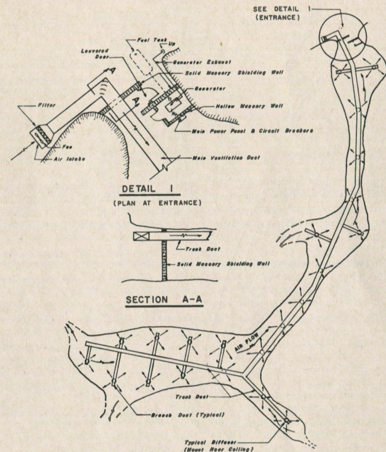
Figure 2 Ventilation system for a cave shelter.
