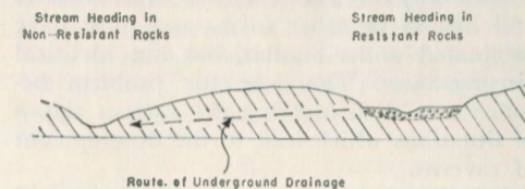
Figure 12 Capture by solution piracy of a stream heading in resistant rocks by a lower stream heading in weakly resistant rocks.
