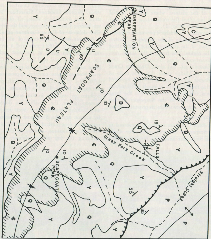
Fig. 3. Geologic map of the Scapegoat area (modified from U.S.G.S. open file map by M. R. Mudge and R. L. Earhart, 1969-1970). Q—Quaternary landslide debris, colluvium, and alluvium. D—Devonian rocks. C—Cambrian rocks. P—Paleozoic rocks (undifferentiated). Y—Pre-Cambrian rocks (undifferentiated).
