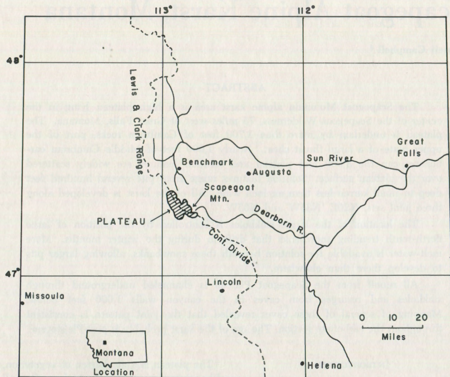
Fig. 1. Index map of northwestern Montana, showing location of Scapegoat Plateau.
