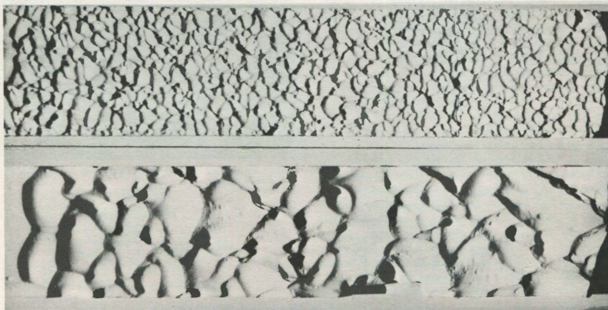
Fig. 3. Artificially produced scallops on plaster of paris, blocks are 76 cm long and 15 cm wide. The larger scallops developed at u (\bar{L}_{22}) = 40 cm/sec and 16^\circ\text{C} ., \bar{L}_{22} = 6.0 cm. The smaller scallops developed at u (\bar{L}_{22}) = 90.7 cm/sec and 33^\circ\text{C} ., \bar{L}_{22} = 1.7 cm. The values of Re_L are both close to 21,000. Flow (and illumination) was from left to right.
