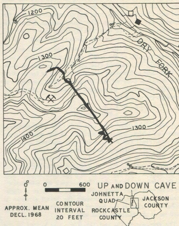
Fig. 1. A portion of the Johnetta 7½ minute quadrangle, showing the location of Up and Down Cave and the relationship of its passages to the land surface above. Note the sink northwest of the entrance and the two springs.
