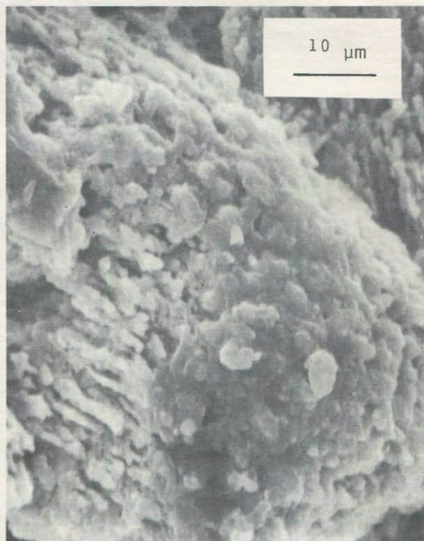
Fig. 6. Scanning electron micrograph of the end of a crystal-like form; note that terminations of individual crystallites are subcircular in cross-section.
