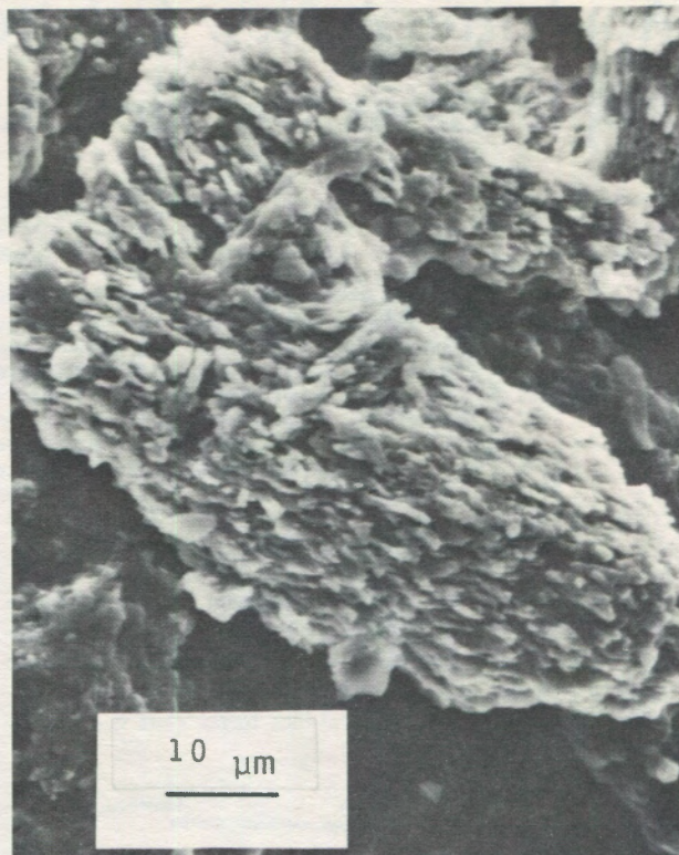
Fig. 4. Scanning electron micrograph of a single crystal-like form, showing its resemblance to a scalenohedron.
