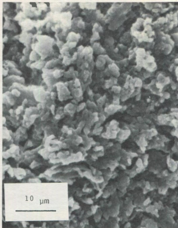
Fig. 8. Scanning electron micrograph of the bottom surface of appelite. Compared with Fig. 6, which is a view of the upper surface, it has a finer texture.
