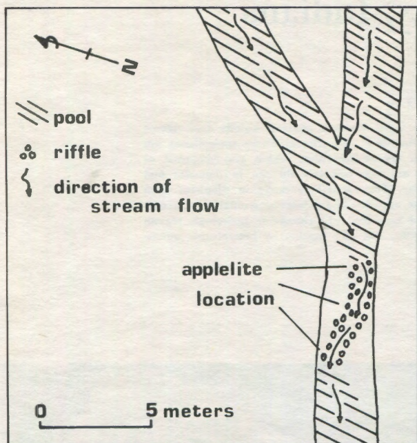
Fig. 3. Map of a portion of Apple Cave, Orange County, Indiana, showing the relationship of Applelite locality to pools and riffles.
