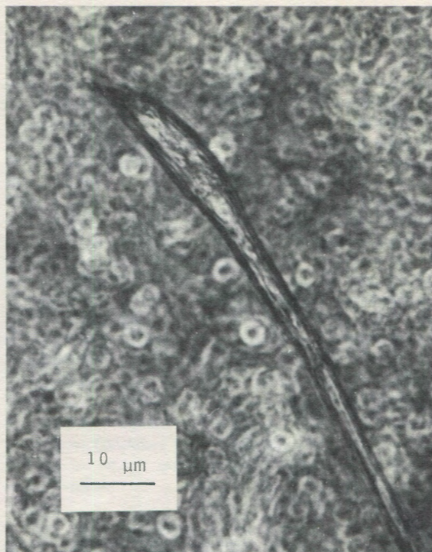
Fig. 12. Photomicrograph, showing the type of bacteria common in the insoluble residue of appelite after EDTA leaching; note dark sheath surrounding ovoid.
