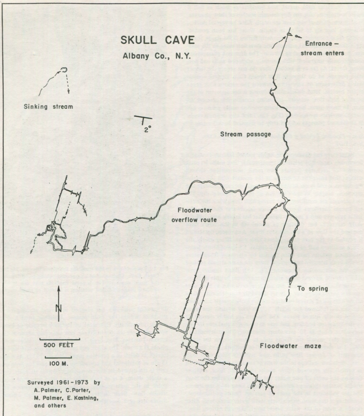
Fig. 13. Map of Skull Cave, New York, showing fissures developed by ponding behind a partially blocked spring. The floodwater passages are confined beneath a shaly cap-rock and have no direct spring outlet (See Palmer, 1962).
