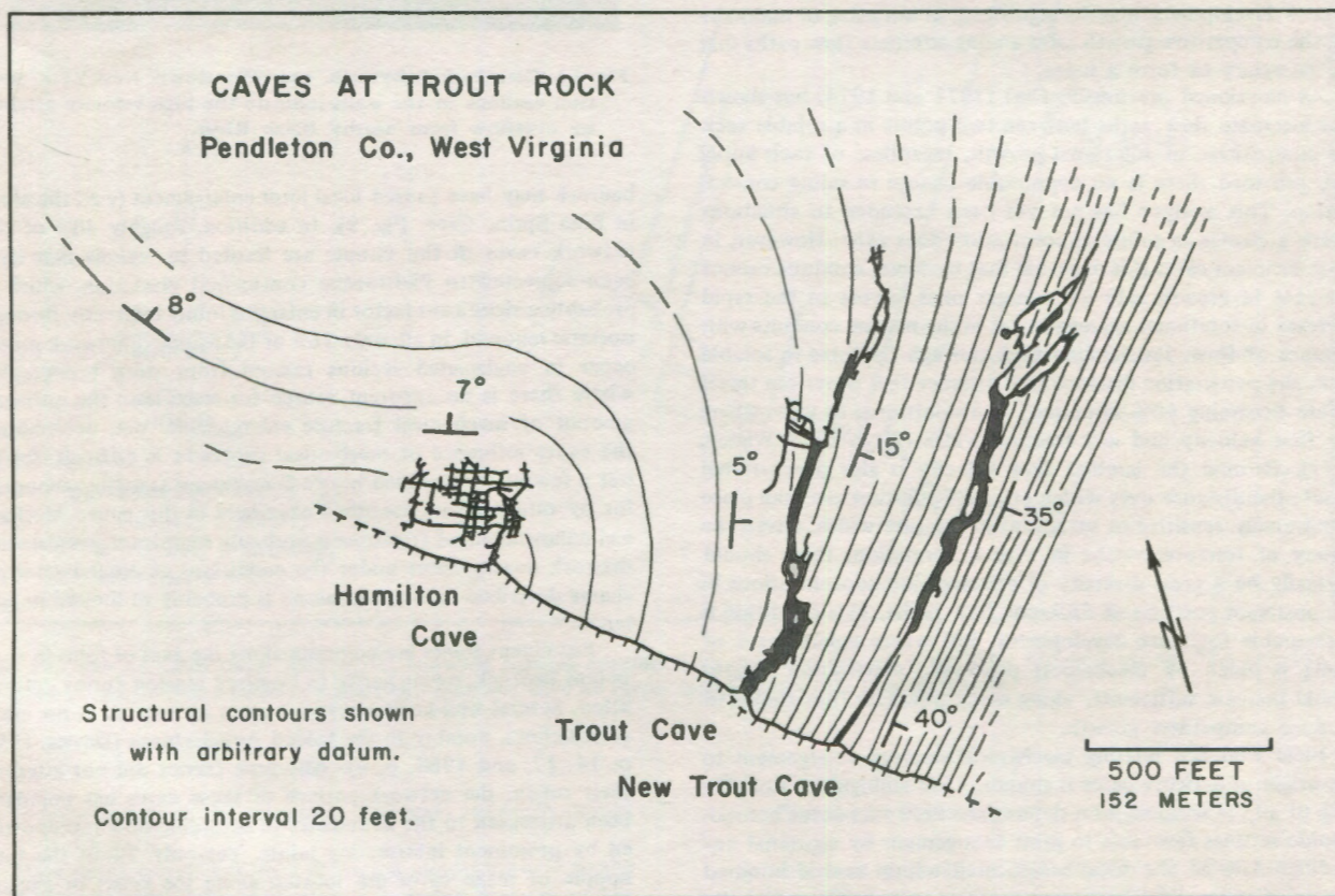
Fig. 15. Structural setting of Hamilton, Trout, and New Trout Caves, West Virginia. Cave maps from Davies, 1958. Structural data by A. Palmer, M. Palmer, J. Allen, and P. Bongei, April, 1969.
