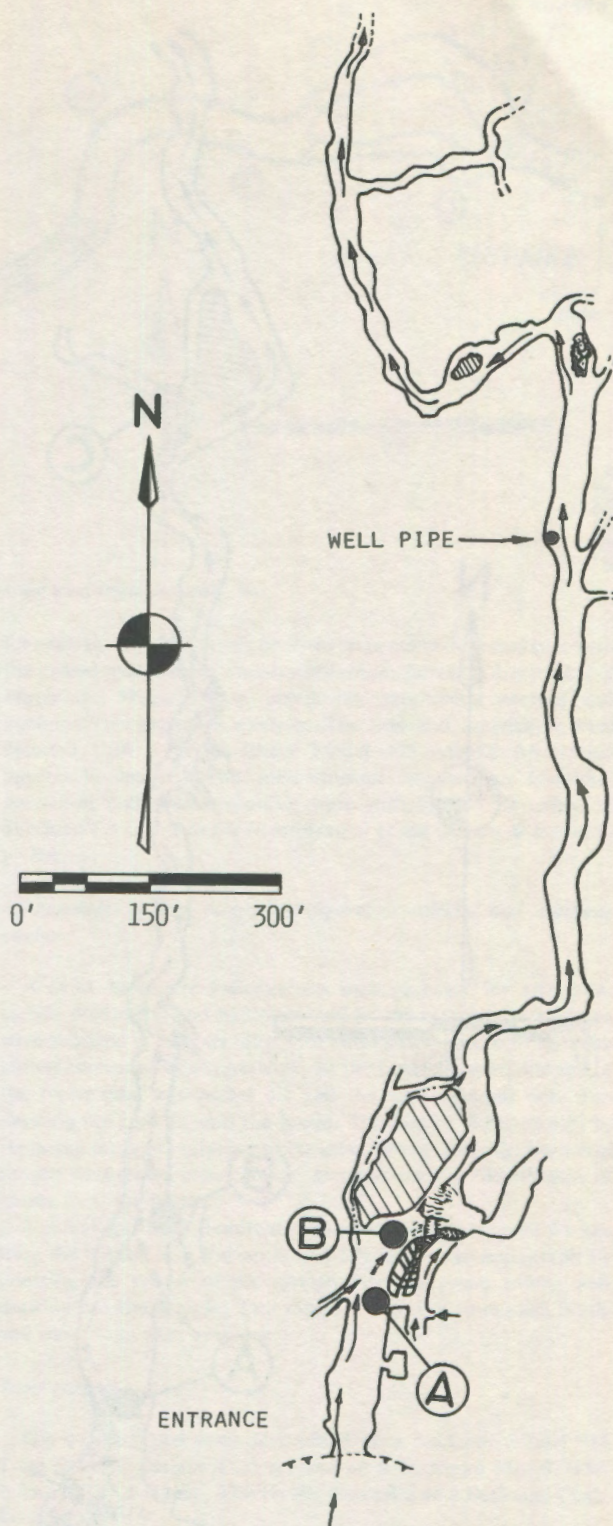
Fig. 3. Map of Lost River Cave.
