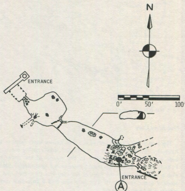
Fig. 6. Map of Lampkin Cave.
