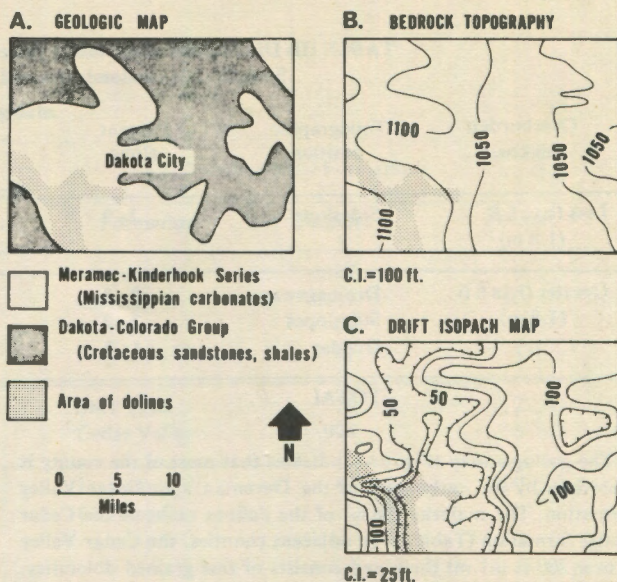
Fig. 9. Doline distribution compared to geology (A), bedrock topography (B), and drift thickness (C). Humboldt County, Iowa (base maps from Hershey, 1969; Palmquist and Bible, 1974).
