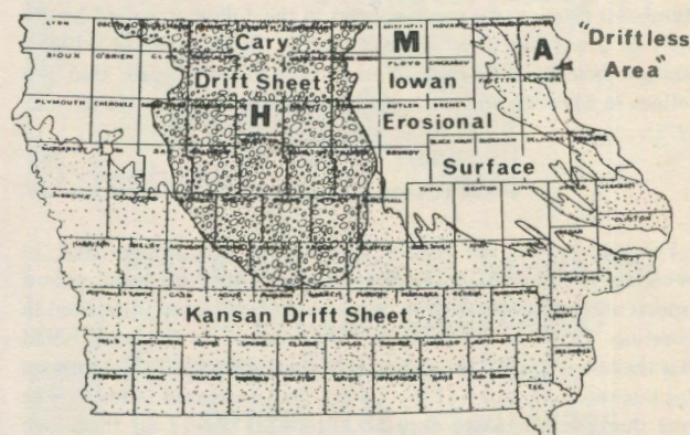
Fig. 1. Index map of Iowa. A = Allamakee County, M = Mitchell County, H = Humboldt County.
