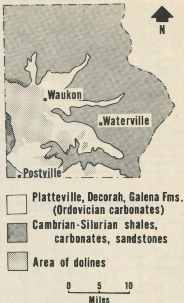
Fig. 3. Geologic map of Allamakee County, Iowa.
