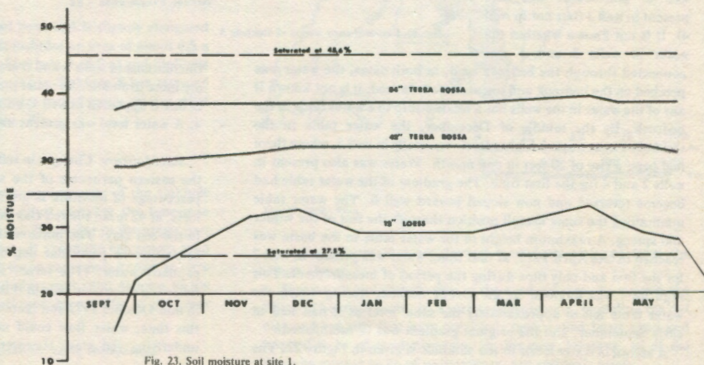
Fig. 23. Soil moisture at site 1.
