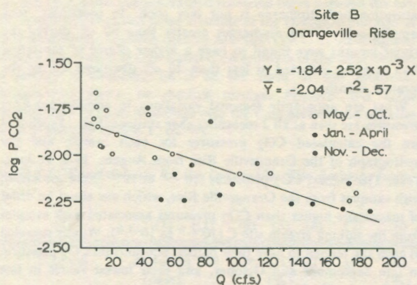
Fig. 12. Graph of P_{CO_2} vs. discharge at the Orangeville Rise.
