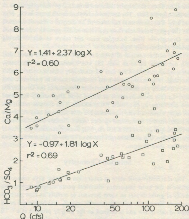
Fig. 14. Graph of Ca/Mg and HCO_3/SO_4 ratios vs. discharge at the Orangeville Rise.
