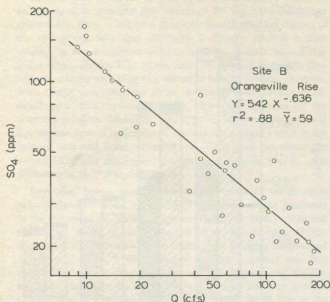
Fig. 9. Graph of \text{SO}_4 vs. discharge at the Orangeville Rise.
