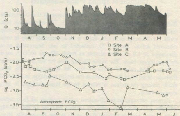
Fig. 11. Diagram illustrating variation in P_{\text{CO}_2} at each of the recording gage stations, plotted with discharge at the Orangeville Rise.
