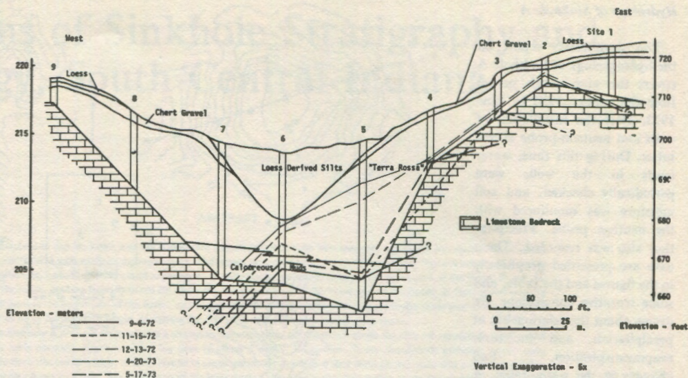
Fig. 21. Sinkhole A water table.
