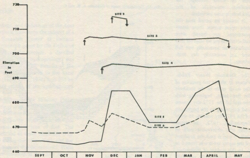
Fig. 22. Water level in Sinkhole A wells.
