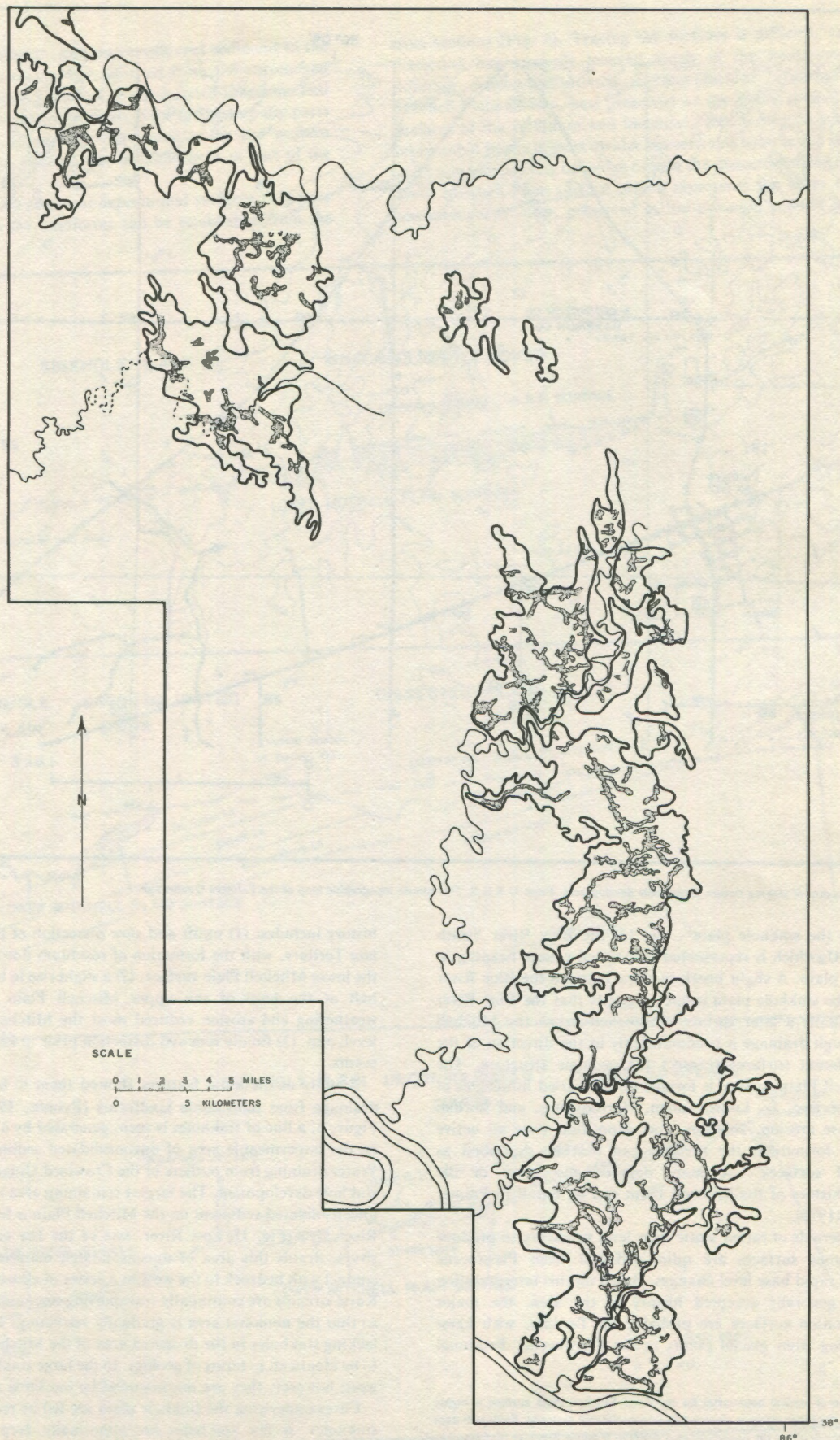
Figure 6. Map of linear zones (stippled) with low sinkhole bottom elevations. Dark lines match boundaries of sinkhole plain development shown on Figure 3.
