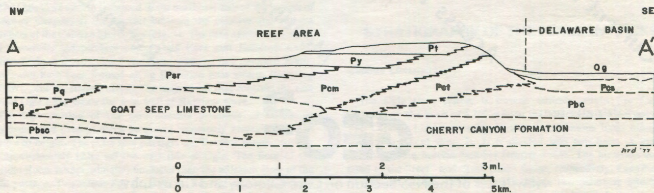
Figure 3. Cross section A-A' through the Capitan Reef complex (see Figure 2). Modified from Hayes, 1964, Plate 3. Units are: Qg = Quaternary Gravel; Permian units are: Pt = Tansill Formation; Py = Yates Formation; Psr = Seven Rivers Formation; Pq = Queen Formation; Pg = Grayburg Formation; Pbse = Bone Springs Formation, Cut Off Shale Member; Pcm = Capitan Limestone, Massive Member; Pet = Capitan Limestone, Reef Talus Member; Pcs = Castile Formation; Pbc = Bell Canyon Formation.
