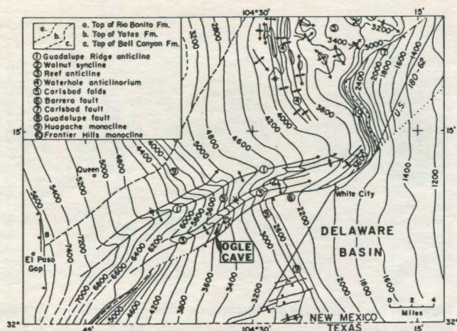
Figure 7. Structural map of the Capitan Reef and adjoining areas (Kelley, 1972, Fig. 3).
