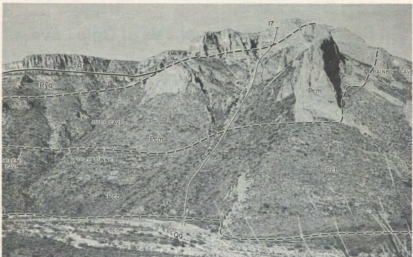
Figure 1. Northeast wall of Slaughter Canyon, showing entrance locations of Ogle Cave, Rainbow Cave, Helen's Cave, and the Ogle tunnel. Lateral transitions of the Yates (Pya) and Tansill (Pt) formations into the massive member of the Capitan Limestone (Pcm) occur directly over Ogle Cave. Ogle and Rainbow caves formed by preferential solution along the transition of the massive member into the breccia member of the Capitan (Pcb). Hayes' stratigraphic section No. 17 (Fig. 4) was measured directly over the cave. Pete Lindsley photo.
