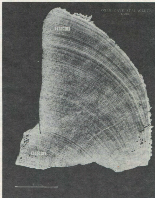
Figure 1. Photograph of the Ogle Cave stalagmite, made from an acetate surface peel. The ^{230}\text{Th}/^{234}\text{U} dated horizons are indicated. Note the equal spacing of growth layers and the more rapid convergence of the topmost growth layer.
