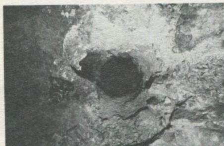
Figure 13. Drip Tube in a gypsum mound in the floor of Upper Kane cave. The carbide lamp has a 10 cm reflector.
