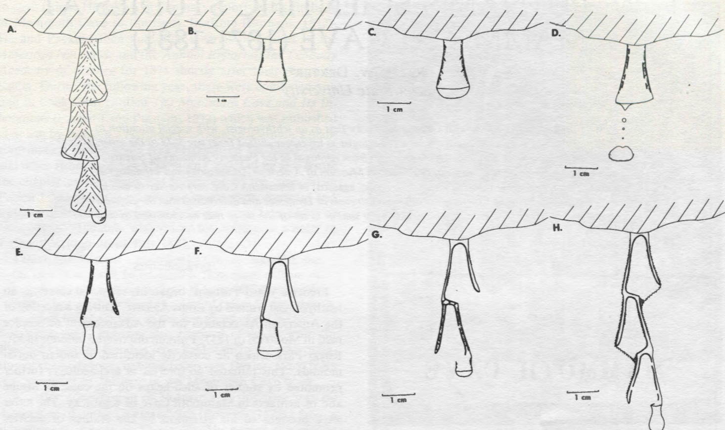
Figure 2. Illustration of idealized phases of spathite development showing external (A) and cross-sectional (B-H) views. A. Stylized multistage aragonite spathite suspended from ceiling. B. Early growth form of an aragonite spathite showing flaring termination. Internal growth of aragonite needles that exhibit a moldy appearance. C. Spathite showing continued flaring; calcite scalenohedrons (bold triangles) associated with aragonite needles. D. Spathite has reached the size where a water drop can only extend across its termination as the drop reaches nearly full size. Growth of a calcite partition (bold internal lines) through the coalescence of a number of segments. E. Spathite has grown to the point where a drop can no longer extend across its termination. A calcite
