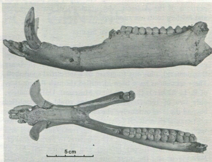
Figure 2. Lower jaw of Mylohyus nasutus from Knob Rock Cave.
