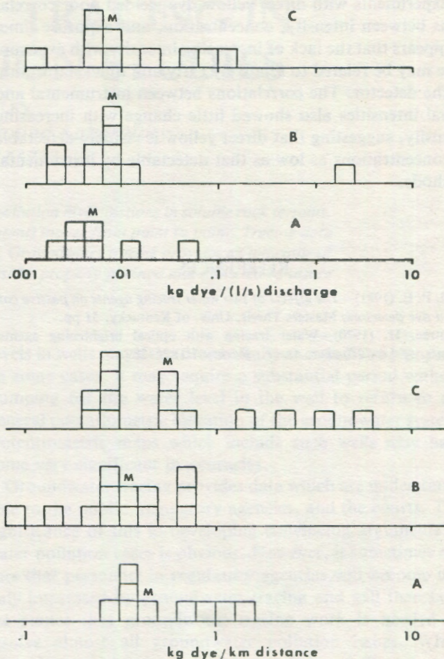
Figure 6. Relationships between visual intensity, dye quantity, spring discharge, and length of trace, for direct yellow dye.
