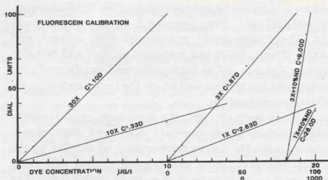
Figure 4. Typical set of calibration curves for fluorescein sodium. Each batch of dye, and each instrument requires a unique standardization to convert the dial readings (or relative fluorescent intensity) to concentration.
