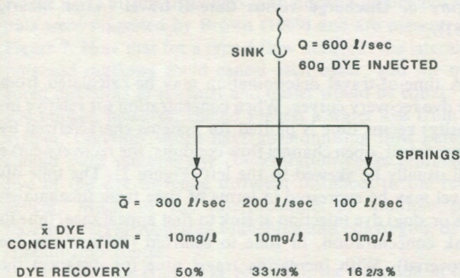
Figure 3. Water budget calculation for a three-way distributory.
