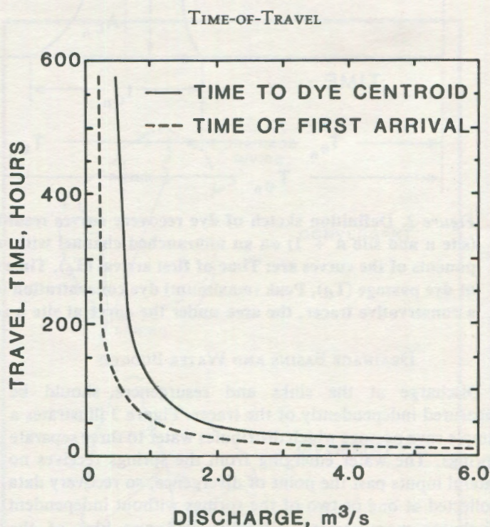
Figure 6. Discharge versus time-of-travel (After Smart, 1981).
