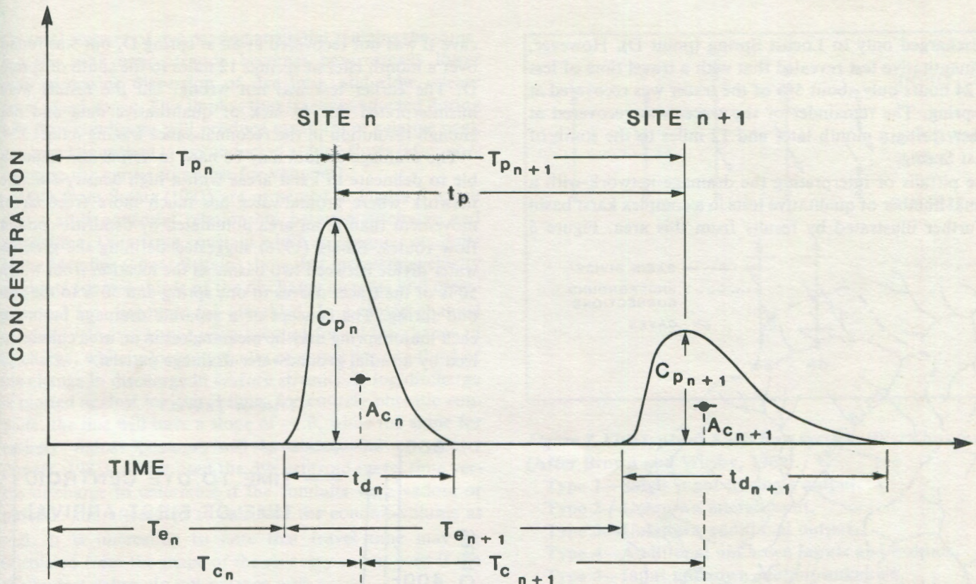
Figure 2. Definition sketch of dye recovery curves resulting from instantaneous dye injection. Two sampling stations (site n and site n + 1 ) on an unbranched channel with no lateral inflows or outflows are shown. The principal components of the curves are: Time of first arrival ( T_e ), Time to peak concentration ( T_p ), Time to centroid ( T_c ), Total Time of dye passage ( T_d ), Peak (maximum) dye concentration ( C_p ), and point representing mean dye concentration ( A_c ). For a conservative tracer, the area under the curve at site n equals the area under the curve at site n + 1 .
