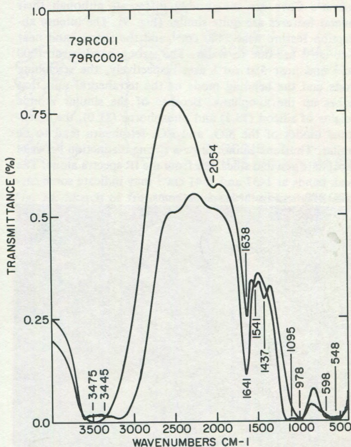
Fig. 9. Infrared spectra for alumino-phosphate white material (79RC002—upper curve) and alumino-silicate white material (79RC011—lower curve).
