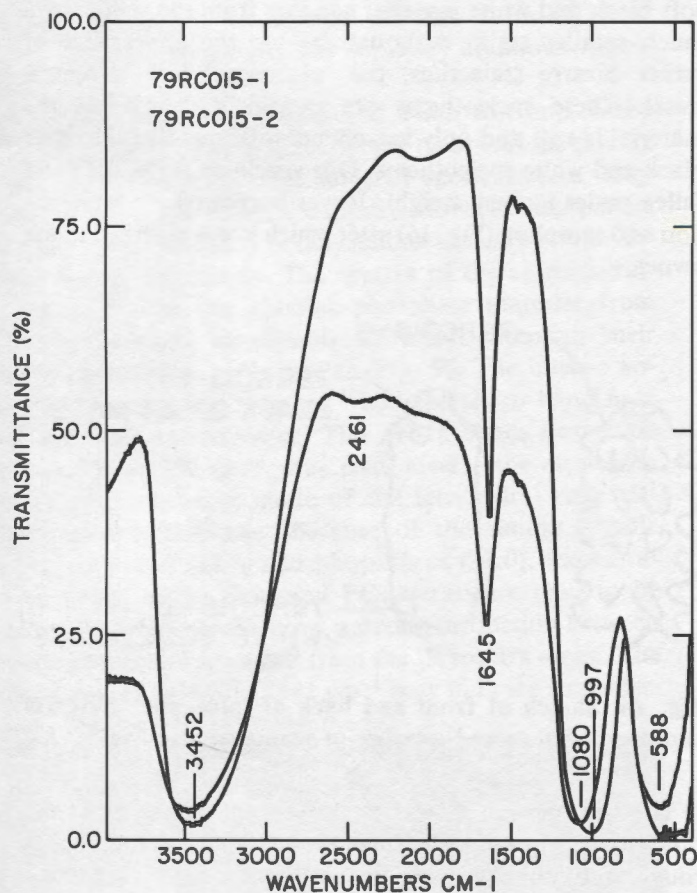
Fig. 17. Infrared spectra of 'pinecone' 79RC015. Split 1 is black material which turns out to be mainly alumina-silica material with some manganese oxide as pigment. Split 2 is alumino-phosphate material.
