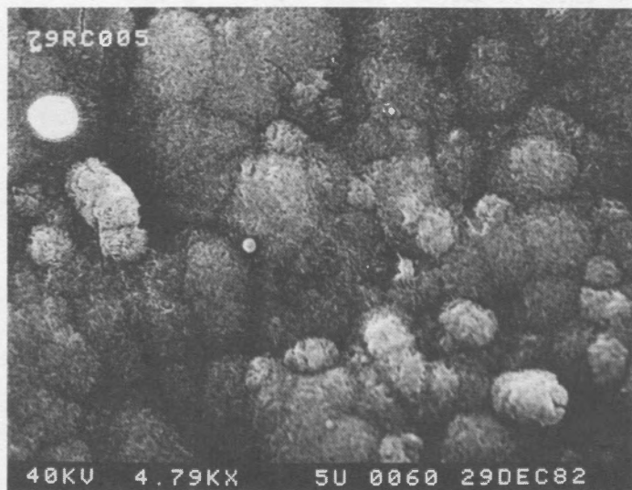
Figure 6. Scanning electron microscope image of limonite stalactite 79RC005 showing nodular and fine platy structure. Image width 22 micrometers.
