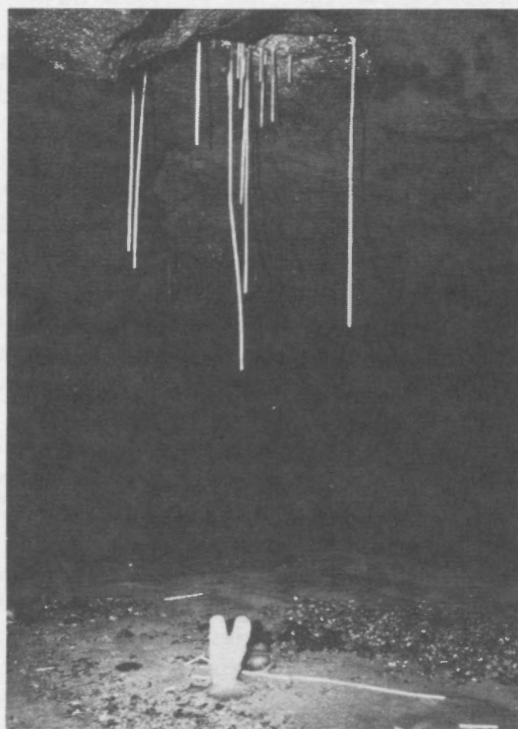
Figure 1. Deflected soda straw with associated stalagmite, Dan-yr-Ogof, South Wales. This is straw #6 in Table 1.
