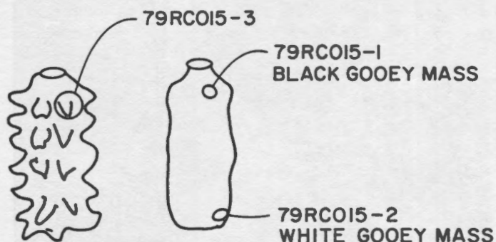
Fig. 16. Sketch of front and back of 'pinecone' 79RC015 showing location and number of extracted samples.
