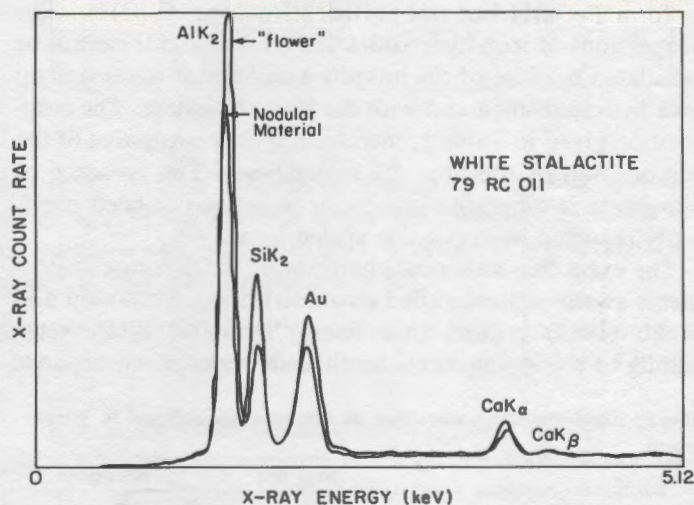
Fig. 12. Energy dispersive X-ray (EDX) spectrum of white stalactite 79RC011. The peak marked 'Au' is an artifact from the gold coating evaporated onto the sample to prevent charging in the electron beam.
