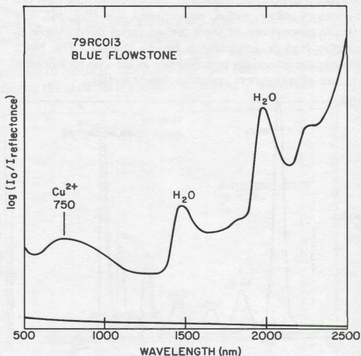
Fig. 19. Diffuse reflectance spectrum of blue flowstone showing characteristic absorption band of \text{Cu}^{2+} .
