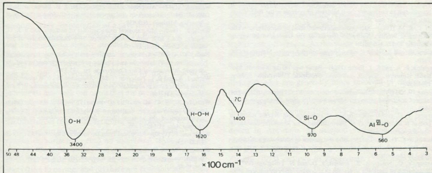
Figure 1. IR absorption spectrum of allophane flowstone from Newton Cave, showing bond assignments for absorption bands.
