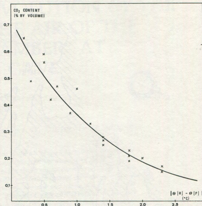
Fig. 3. CO 2 content in the air of the Paintings Chamber as a function of the absolute value of the temperature difference between the Hall Chamber and the Paintings Chamber.
