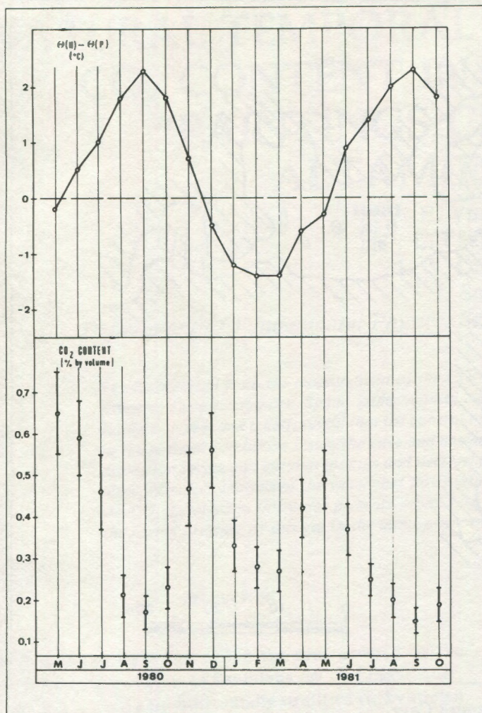
Fig. 2. Annual variations of the average monthly CO 2 content in the Paintings Chamber and of the temperature difference between the Hall Chamber and the Paintings Chamber.
