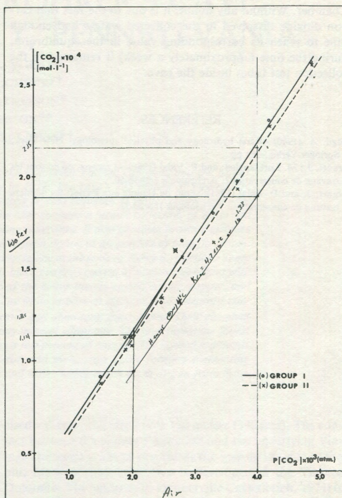
Fig. 4. CO 2 content dissolved in the waters flowing to the Paintings Chamber as a function of its partial pressure in the air.
