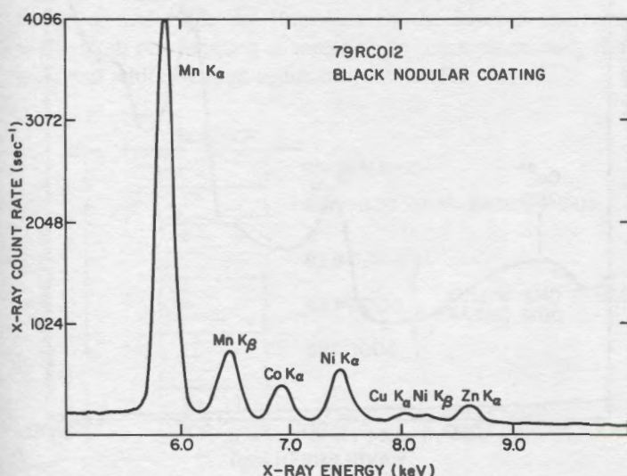
Fig. 14. EDX spectrum of black manganese-rich nodule showing mixture of transition metals present. Concentrations are roughly proportional to peak count rates.
