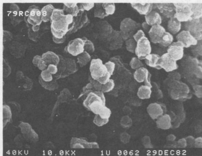
Fig. 23. SEM image of white layers in the gray-white banded sediment 79RC008. Image width 12 \mu\text{m} .
