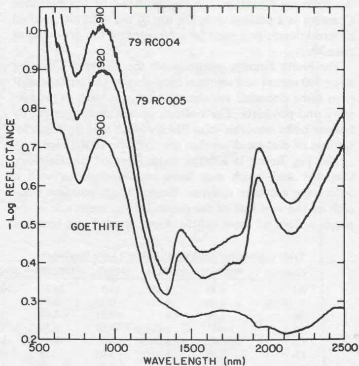
Figure 7. Diffuse reflectance spectra of limonite speleothems in comparison with crystalline goethite. 79RC004 is an orange stalactite. 79RC005 is a nearly black stalagmite similar to those in Figures 2 and 3.
