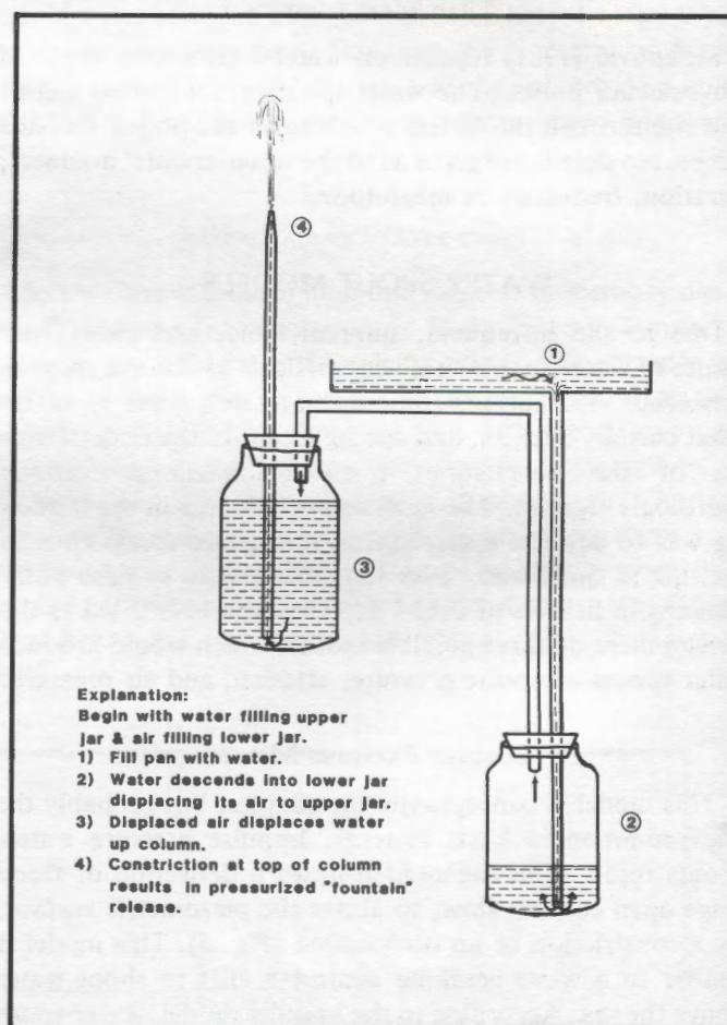
Figure 8. Hero's Fountain.
