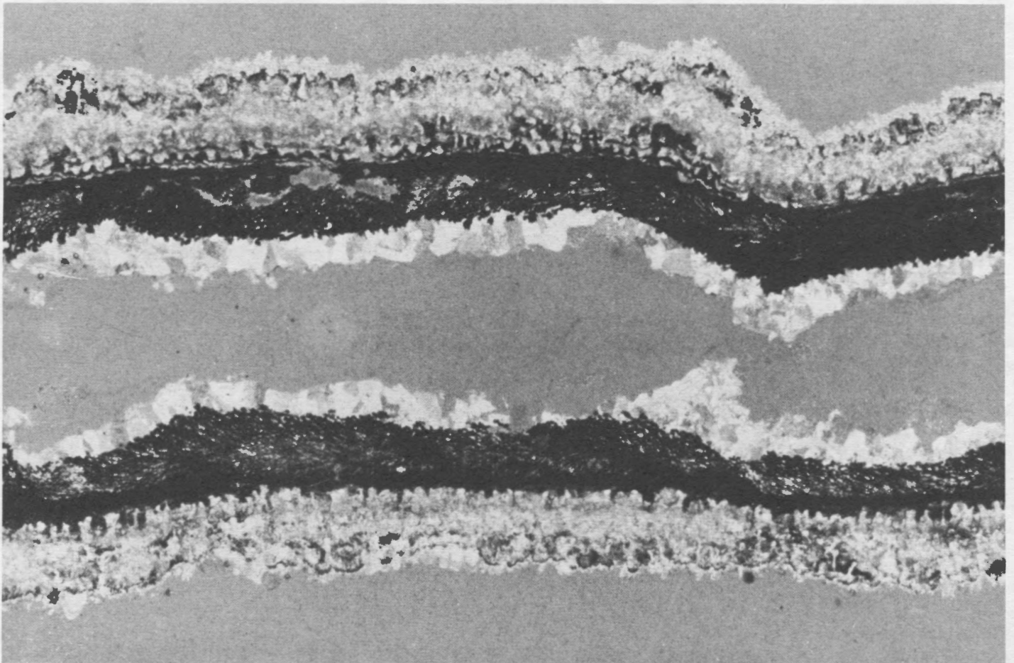
Figure 16. Thin section of an iron-oxide-rich soda straw stalactite at site O in Figure 1. Diameter = 5 mm. The iron oxide, which forms the dark layer, coats a tangle of organic filaments. That layer is coated both inside and out by calcite. (M. Palmer.)
