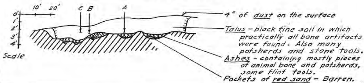
Section I-I Profile of Productive Excavation (Vertical scale exaggerated)
