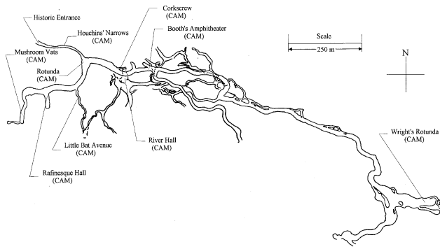
Figure 1. Cave atmospheric monitoring (CAM) stations in the Historic Section of Mammoth Cave (modified after Kaemper 1908).
