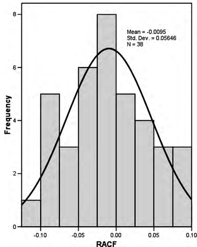
Figure 7. Plot of the residuals (RACF) of ARIMA(1,0,1)(0,1,1)_{12} monthly model with normal curve.
