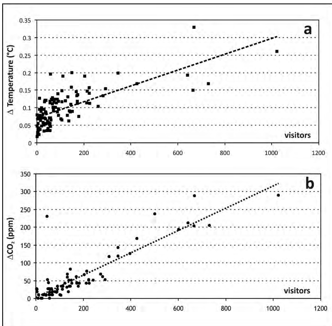
Figure 6. Relation between daily visits and net increase in T_{int} (a) and CO_2 concentration (b) calculated during periods without cumulative effect.
