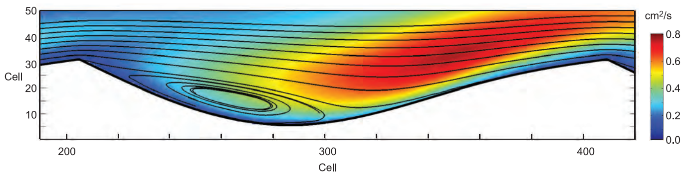
Figure 2. The central part of the modeled domain, with mean-field flow streamlines (black). The eddy viscosity field (colors) indicates degree of local turbulence.
