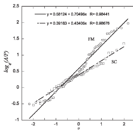
Figure 1. Log-normal probability plots of area/perimeter ( A/P ) data for flank margin caves (FM) and San Salvador sea caves (SC), from Waterstrat (2007). Z is the standard unit-normal variable corresponding to the estimated cumulative probability for each data point.
